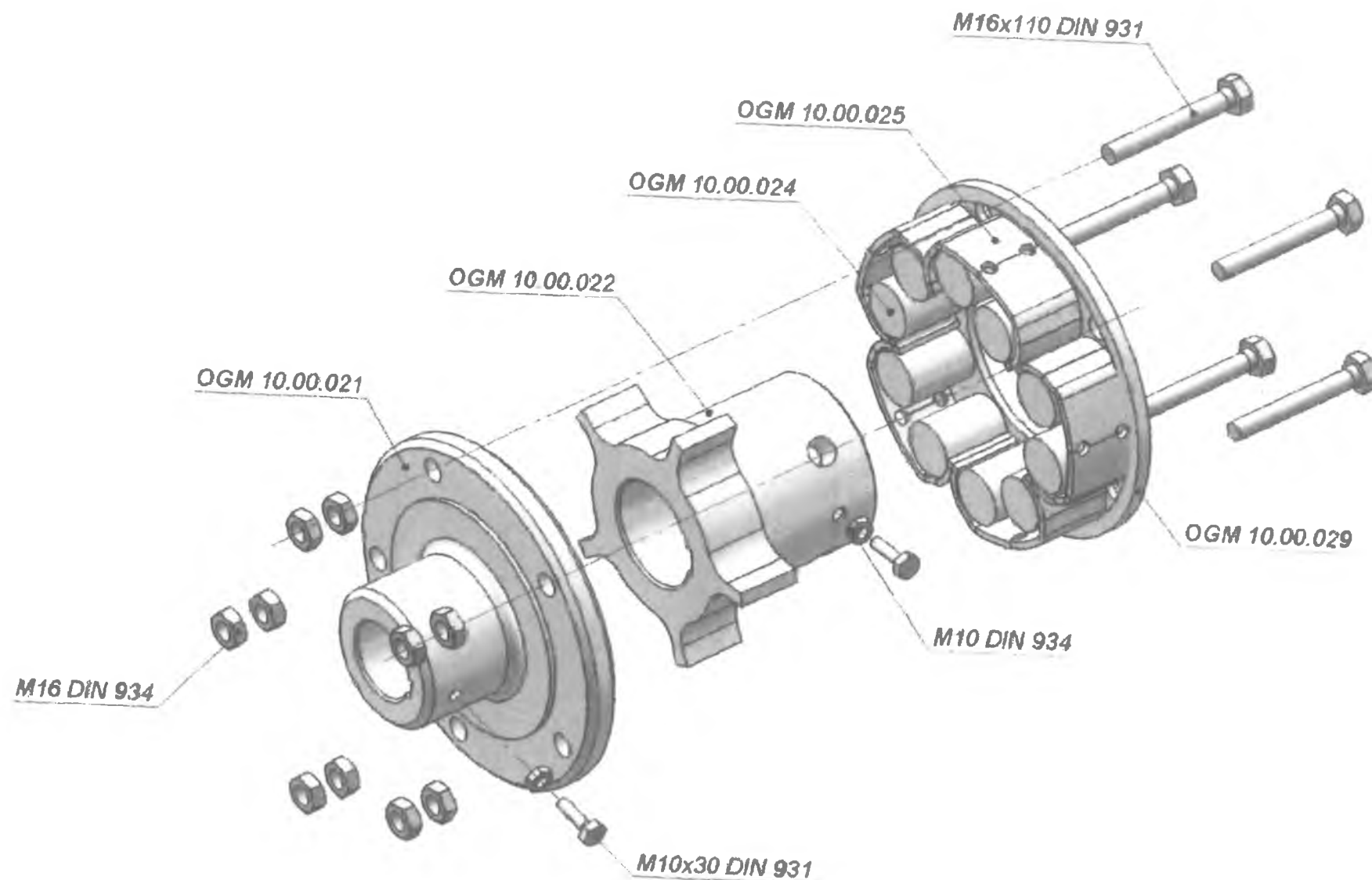
Pav. 2. Mova (OGM 10.00.020) Pic. 2. Coupling Рис. 2. Муфта
